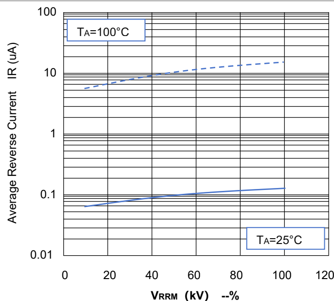
Reverse Characteristics
