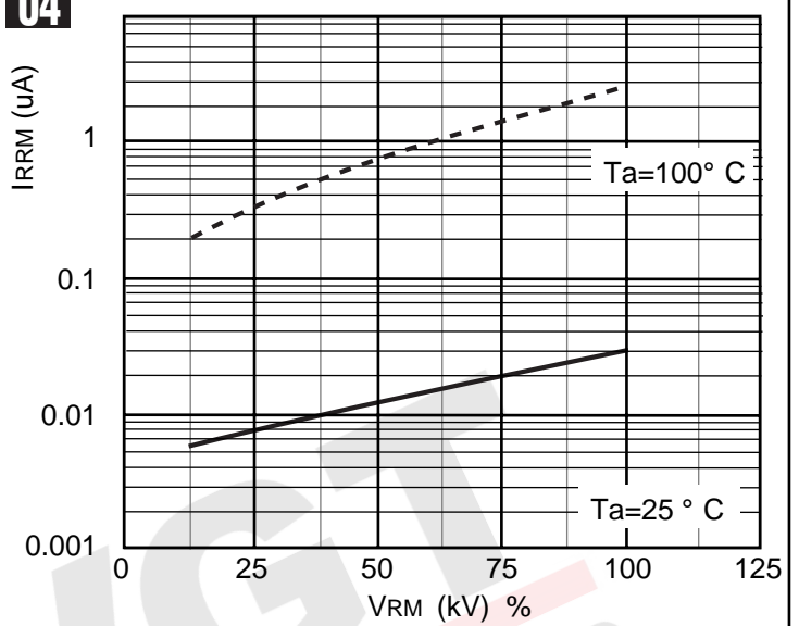
FIGURE 04 Reverse Characteristics
