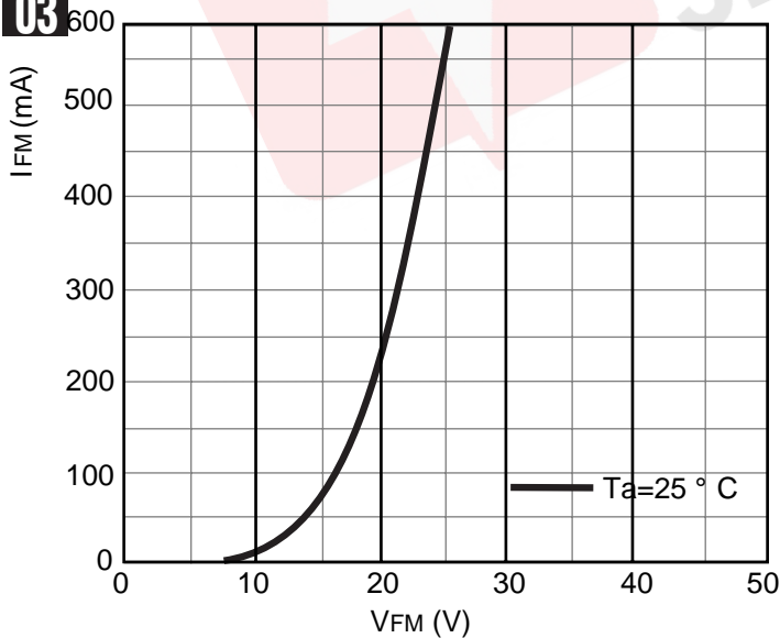
FIGURE 03 Forward Characteristics
