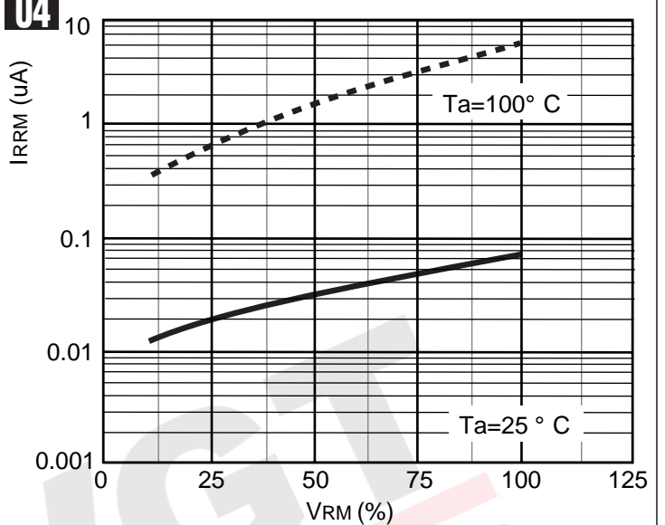
FIGURE 04 Reverse Characteristics
