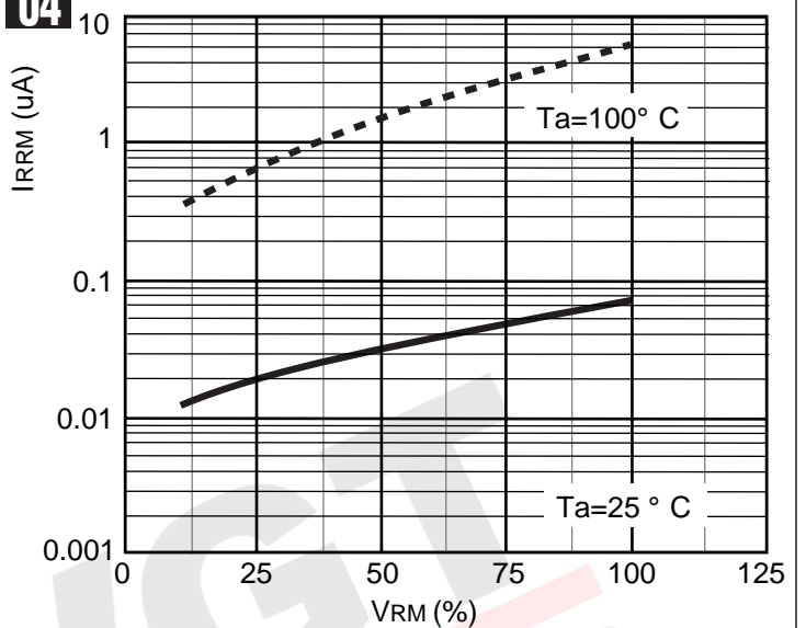
FIGURE 04 Reverse Characteristics
