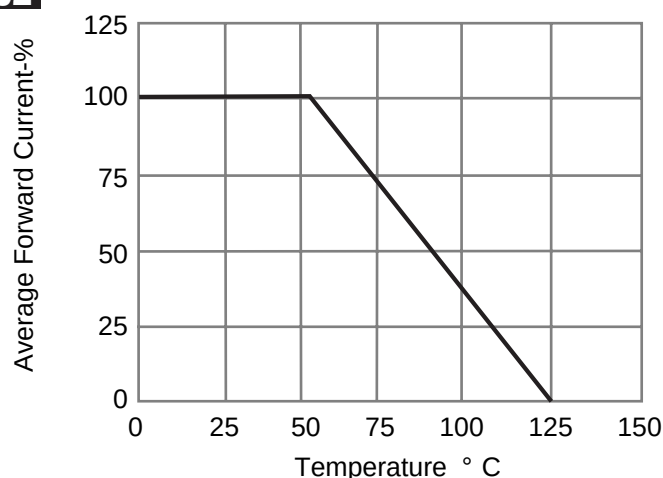
FIGURE 02 Forward Current Derating Curve
