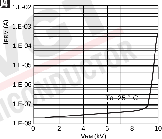
FIGURE 04 Reverse Characteristics
