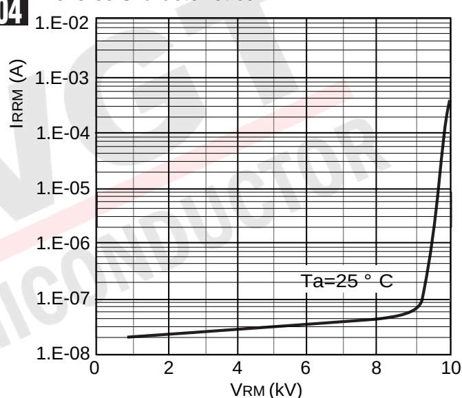
FIGURE 04 Reverse Characteristics
