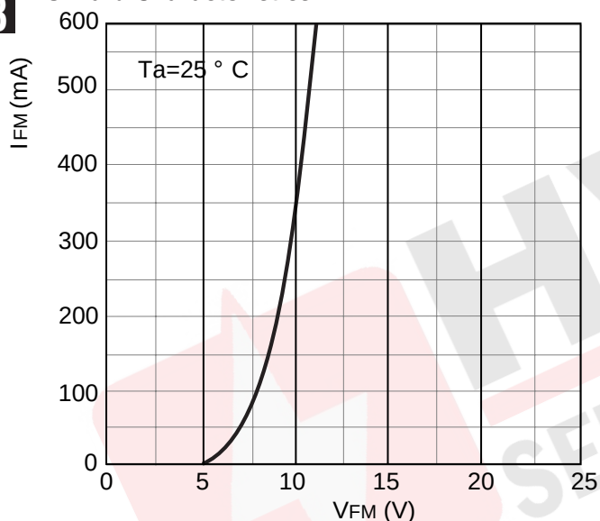
FIGURE 03 Forward Characteristics
