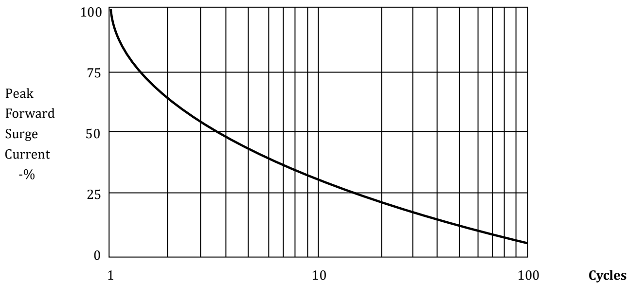
Non-Repetitive Surge Current
