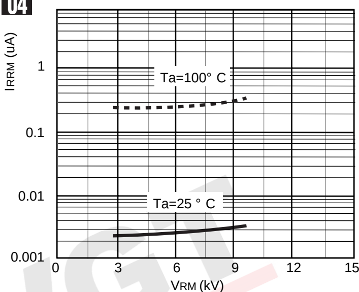
FIGURE 04 Reverse Characteristics
